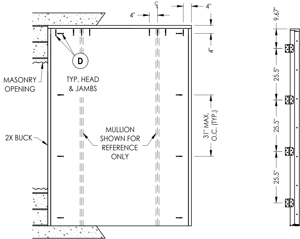
BUCK ANCHORING
