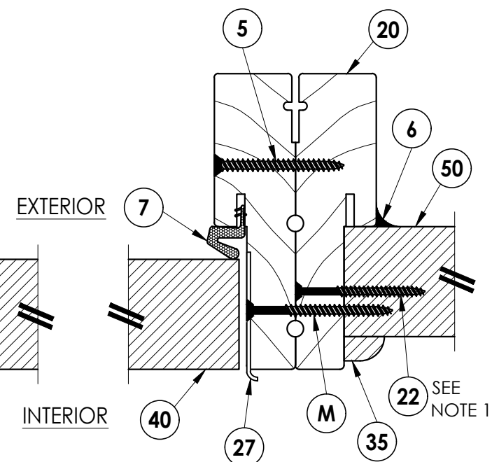
5/4 HORIZONTAL CROSS SECTION
