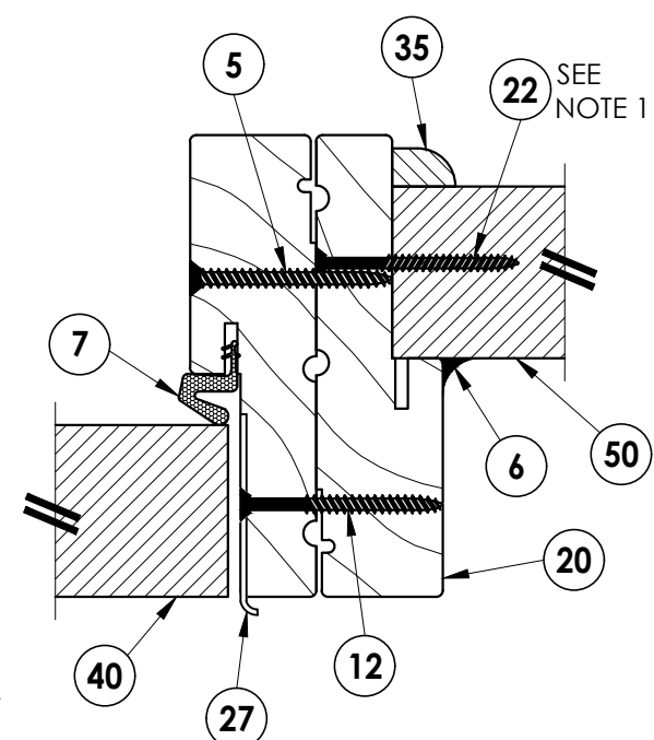
3 HORIZONTAL CROSS SECTION
