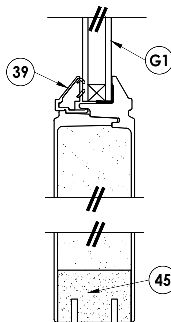
2 2 VERTICAL CROSS SECTION
